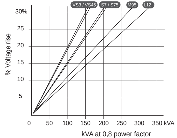
Motor starting (AREP ou PMG excitation)
