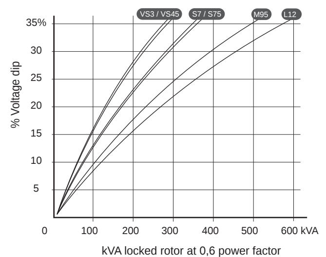
Motor starting (AREP ou PMG excitation)
